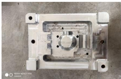
Job Work Machining on Core Insert Plate
